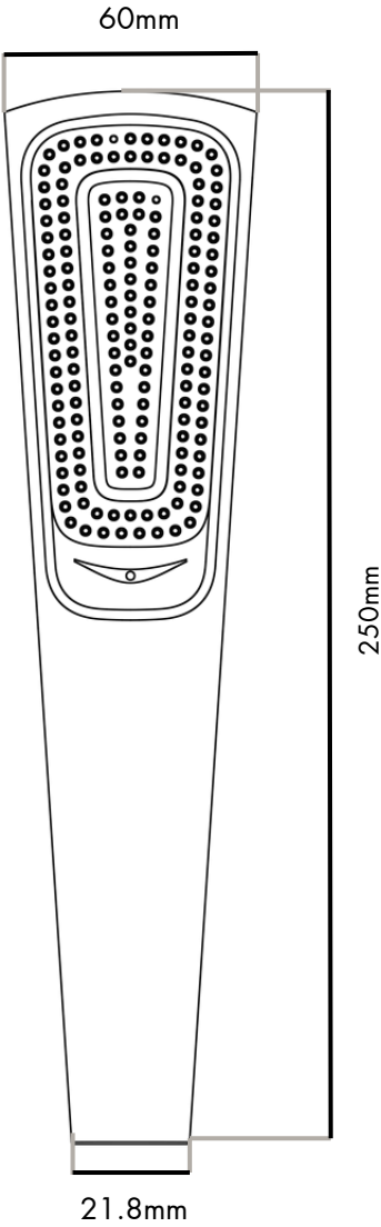
FRONT VIEW
