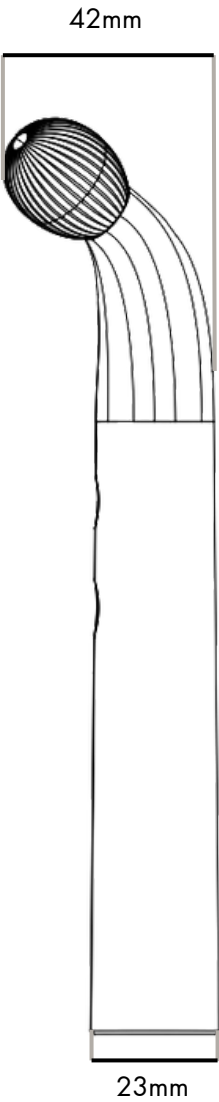
SIDE VIEW
