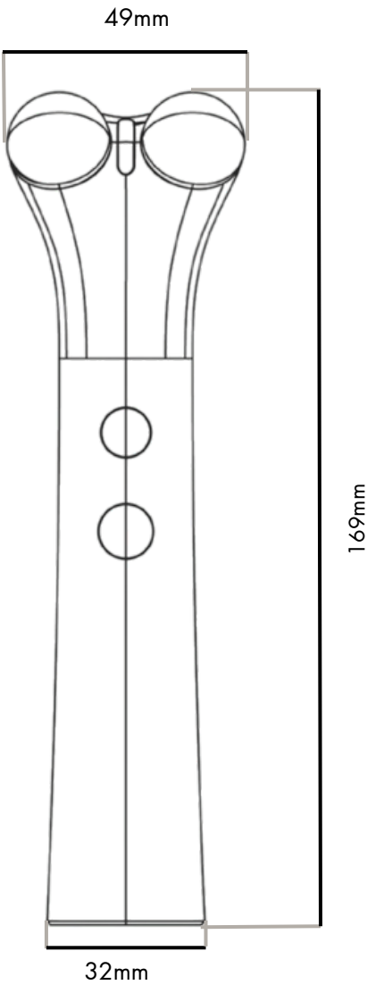
FRONT VIEW
