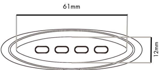
TOP VIEW OF MASSAGE HEAD CONTACT SURFACE
