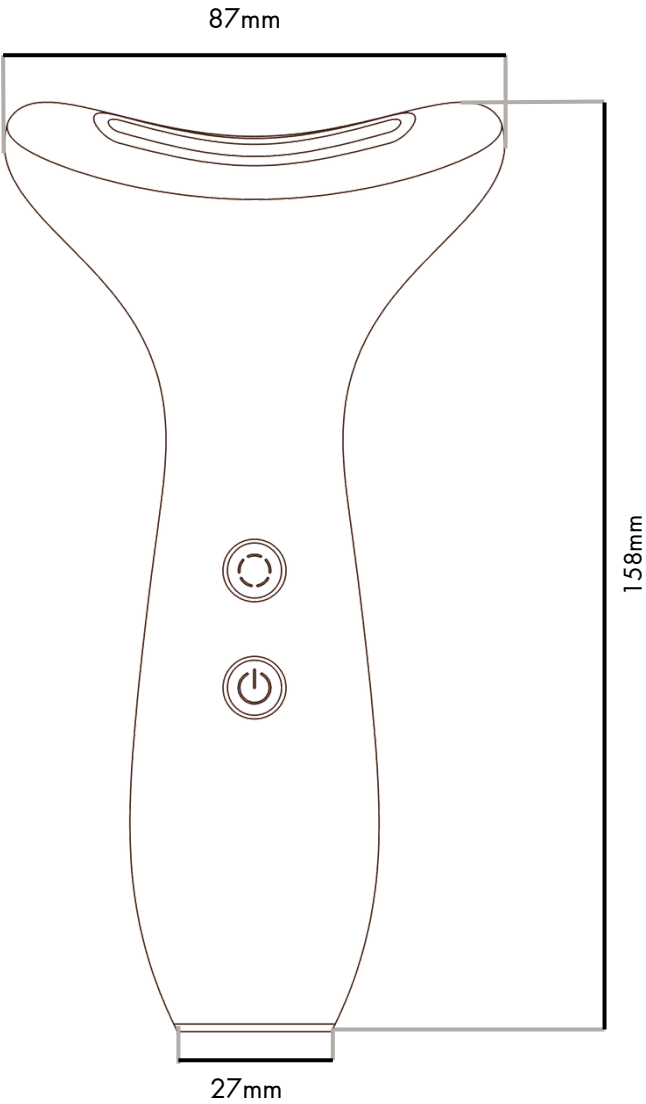
FRONT VIEW
